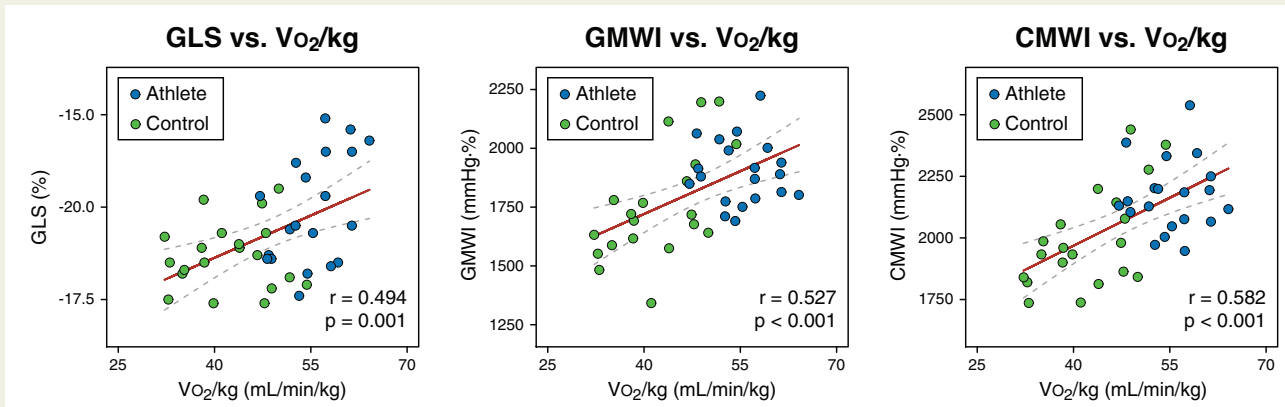
Figure 5 Correlations between peak oxygen uptake and left ventricular deformation parameters in human athletes. CMWI, constructive myocardial work index; GLS, global longitudinal strain; GMWI, global myocardial work index; VO_2/kg , peak oxygen uptake.
